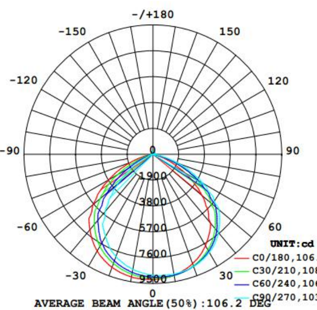
Luminance Intensity Distribution
