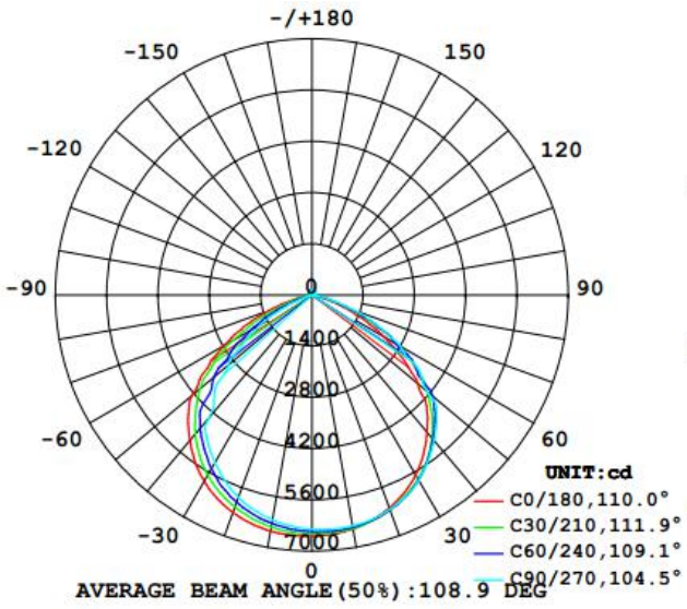
Luminance Intensity Distribution
