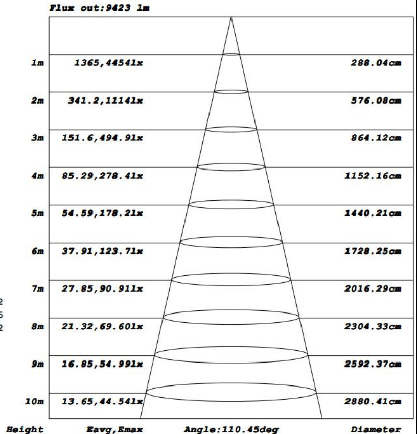
Cone Lux Diagram
