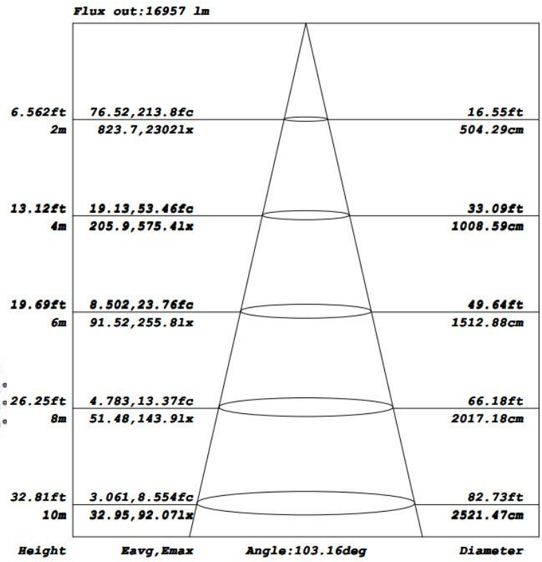
Cone Lux Diagram
